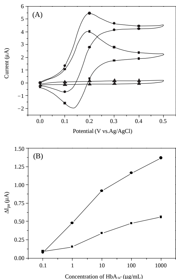
Figure 6. Bio-electrocatalyzed signal amplification using a GOX-modified electrode. (A) Cyclic voltammograms from different solution conditions: in the presence of HbA 1C , non-labeled (up triangle), in the presence of HbA 1C -FcBA conjugate and without glucose (square), and in the presence of HbA 1C -FcBA conjugate and 10 mM glucose (circle). (B) Signal comparisons according to the concentration of HbA 1C . Calibrations from amplified mode (circle) and unamplified mode (square) are shown.
