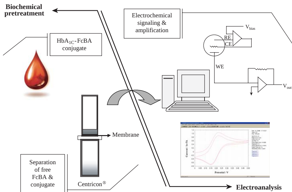
Figure 2. Schematic overview of the HbA 1C detection method, divided into a biochemical pretreatment and electroanalysis processes.
