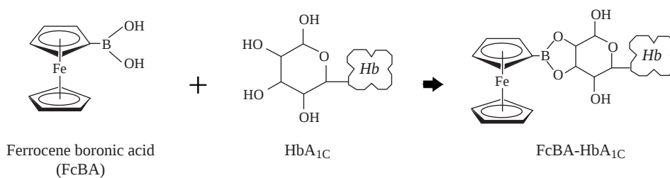
Figure 1. Biospecific covalent bonding between FcBA and HbA 1C .
