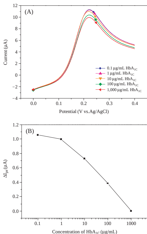
Figure 3. Electrochemical analysis of the free (unreacted) FcBA. (A) Voltammetric results from different HbA 1C concentrations. The concentration of FcBA was fixed at 0.5 mM. (circle) 0.1 μg/mL HbA 1C , (up triangle) 1 μg/mL HbA 1C , (down triangle) 10 μg/mL HbA 1C , (diamond) 100 μg/mL HbA 1C , (left triangle) 1,000 μg/mL HbA 1C , (B) Background-subtracted anodic peak currents from respective voltammograms.
