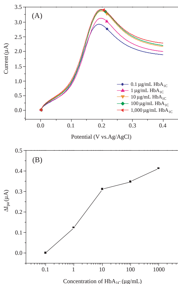
Figure 4. Electrochemical analysis of the HbA 1C -FcBA conjugate. (A) Voltammetric traces registered from samples with different HbA 1C concentrations. (circle) 0.1 μg/mL HbA 1C , (up triangle) 1 μg/mL HbA 1C , (down triangle) 10 μg/mL HbA 1C , (diamond) 100 μg/mL HbA 1C , (left triangle) 1,000 μg/mL HbA 1C . (B) Background-subtracted anodic peak currents from respective voltammograms.
